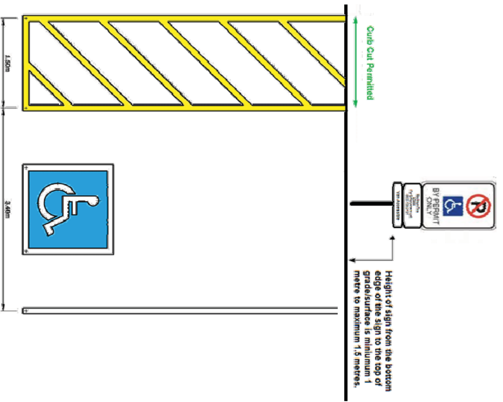
Sign Placement – Single Space
